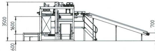
Side view of PIKOMAT HDQ-Compact
