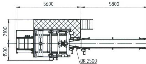
Top view of PIKOMAT HDQ-Compact
